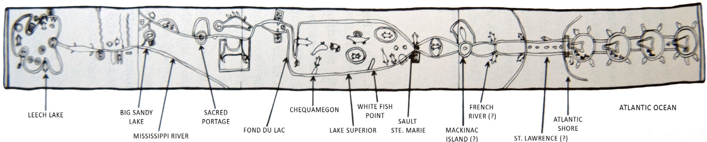
Red Sky's migration chart. (Drawing by B. Nemeth. Courtesy of the University of Toronto Press, Glenbow Museum.)
